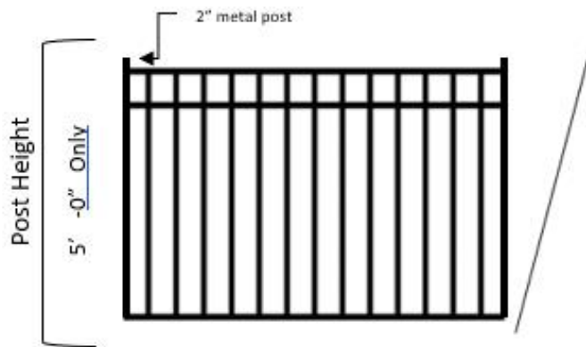
Straight Topped Wrought Iron or Aluminum Fence
