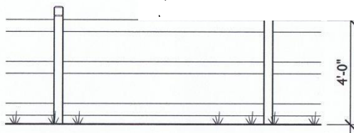
Fence #1: 5/4" x 6" Rail Fence Welded wire mesh "hog wire" optional on inside face.
