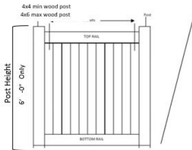
Capped Privacy Fence
