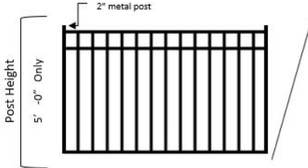
Straight Topped Wrought Iron or Aluminum Fence
